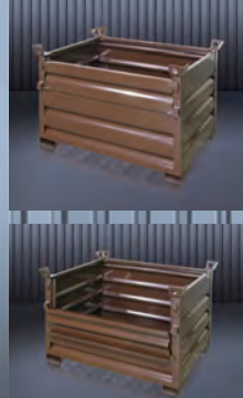
1322.5-8+11 One drop side 1/3 (long side)
